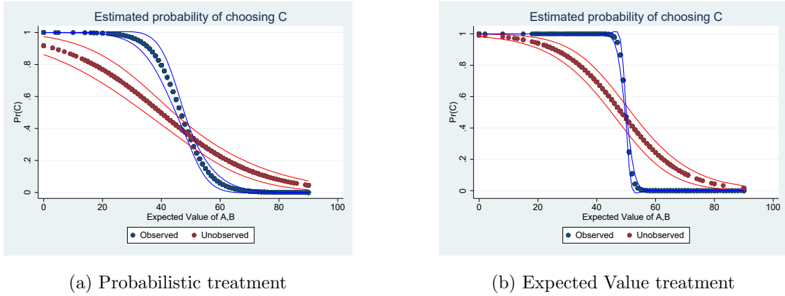
Figure 3: Estimated (logit) driver choice probabilities, with 95% confidence intervals.
